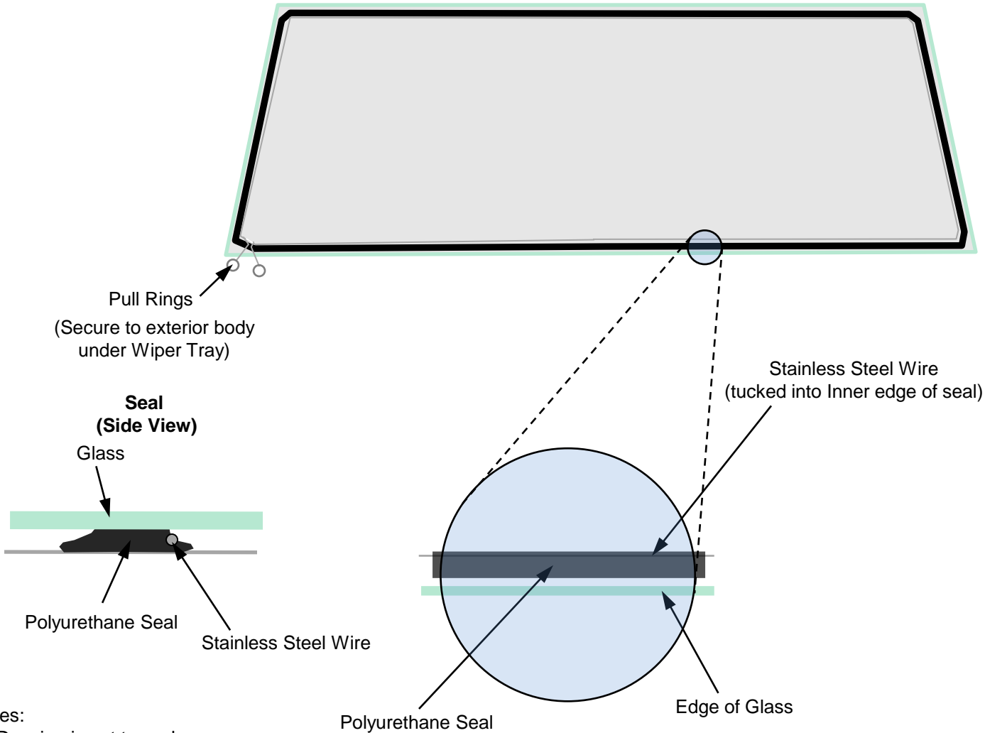
Front Glass (Inside View)
